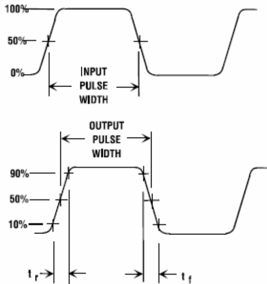
FIGURE 6: SWITCHING WAVEFORM
